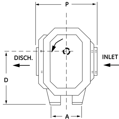
VERTICAL CONFIGURATION (Horizontal Air Flow)
