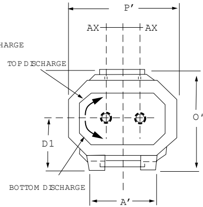
HORIZONTAL CONFIGURATION (Vertical Air Flow)
